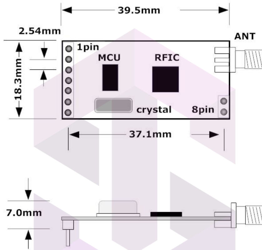
Figure 4: Mechanical dimension
